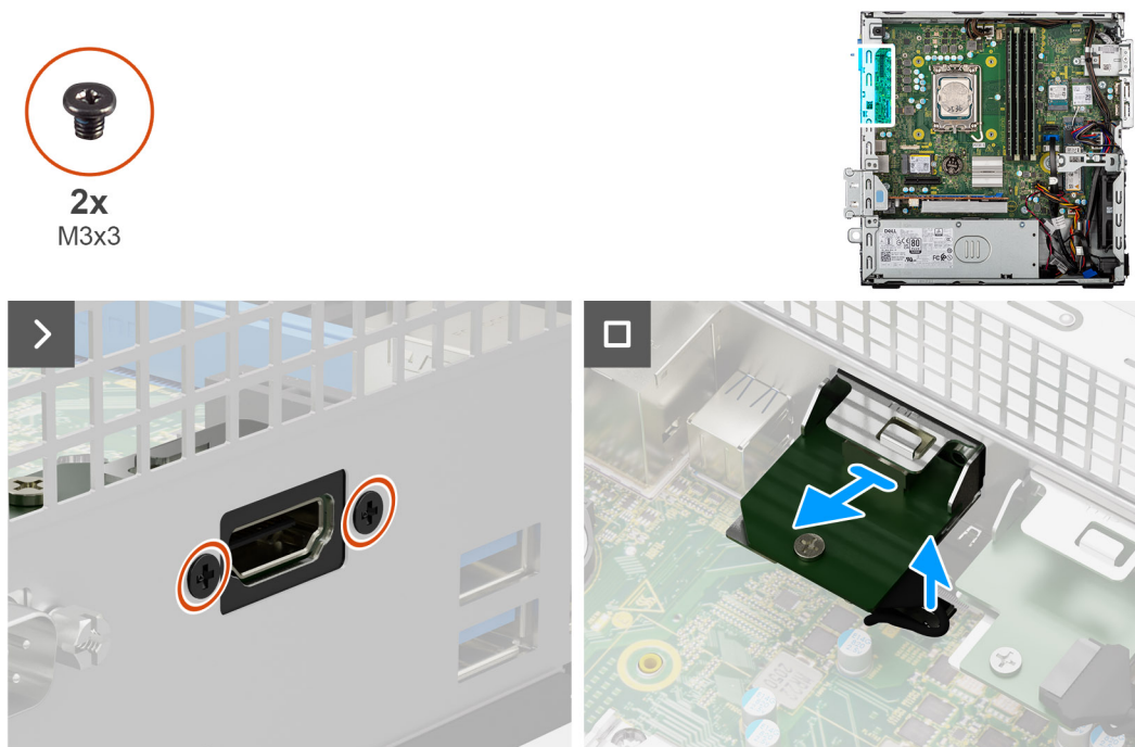
Figure 58. Removing the HDMI module
