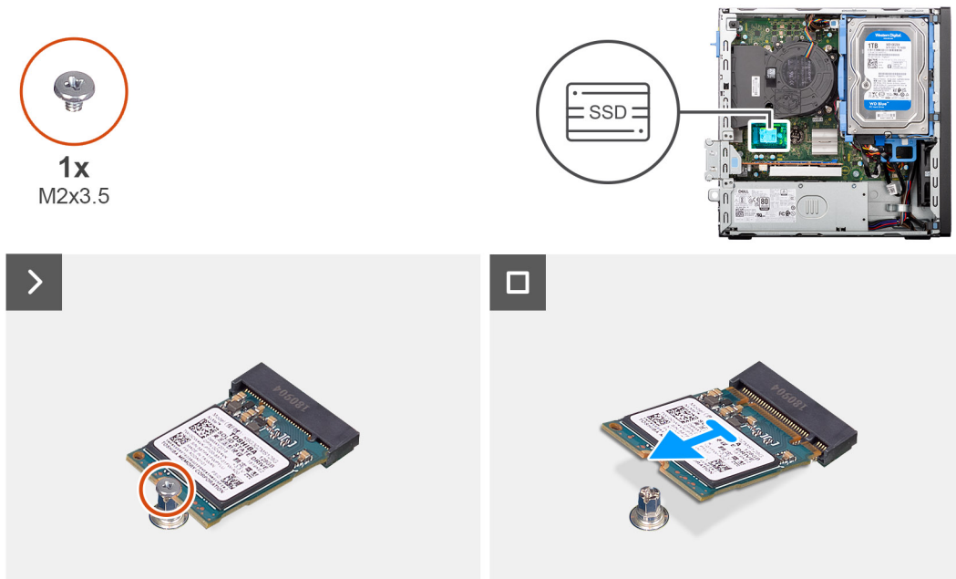
Figure 17. Removing the M.2 2230 solid-state drive
